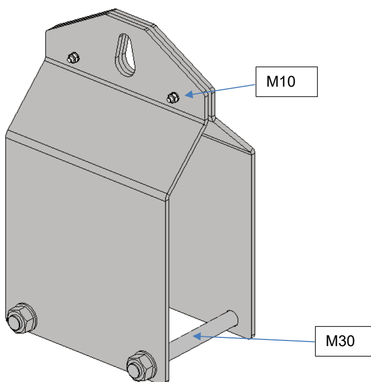
Figure 3: Lifting device in detail.
