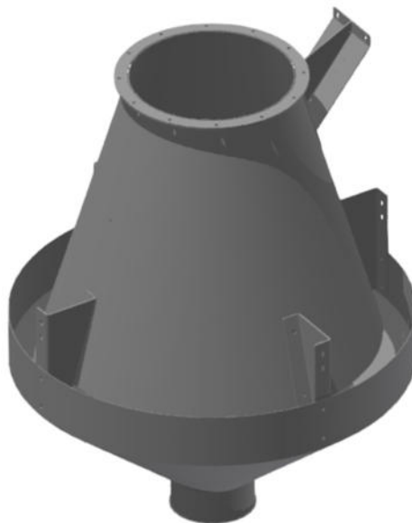
Figure 4: Lower part
